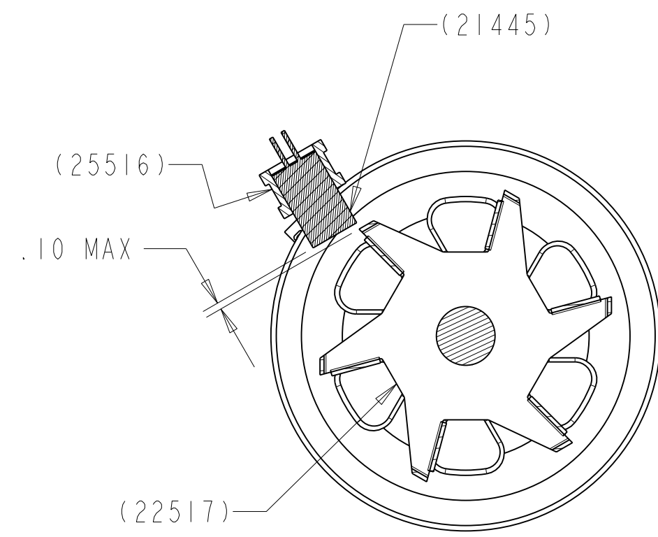
SECTION B-B
